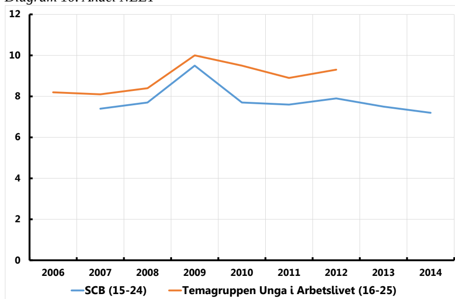
Diagram 10. Andel NEET
