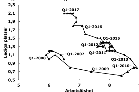
Diagram 19. Beveridgekurvan
